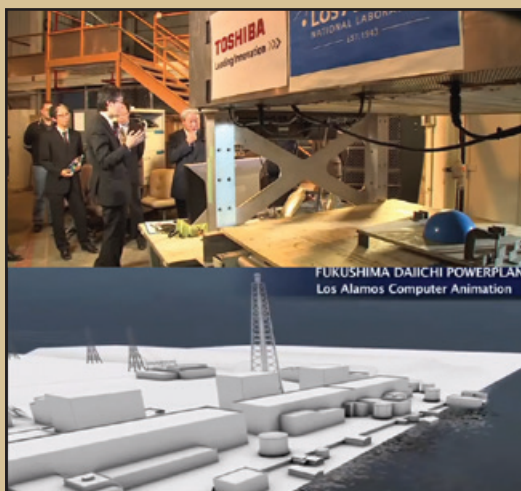
Los Alamos is partnering with Toshiba Corporation to use a Los Alamos technique called muon tomography to safely peer inside the cores of the Fukushima Daiichi reactors and create high-resolution images of the damaged nuclear material inside without ever breaching the cores themselves.
